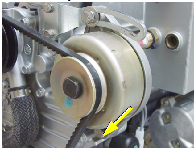
Fig. 7.9-2: Lichtmaschine
