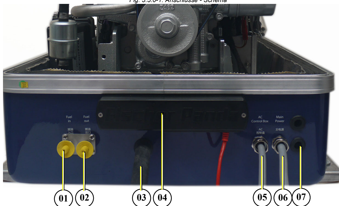
Fig. 5.5.0-1: Anschlüsse - Schema
