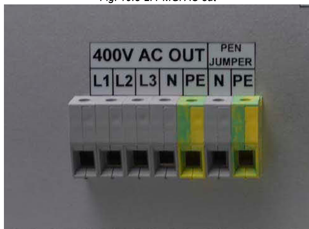
Fig. 19.5-3: PMGi AC out
