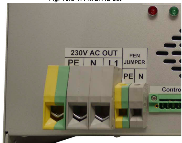
Fig. 19.5-1: PMGi AC out
