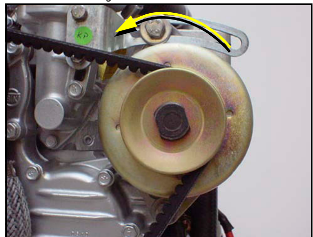
Fig. 9.15-3: Lichtmaschine
