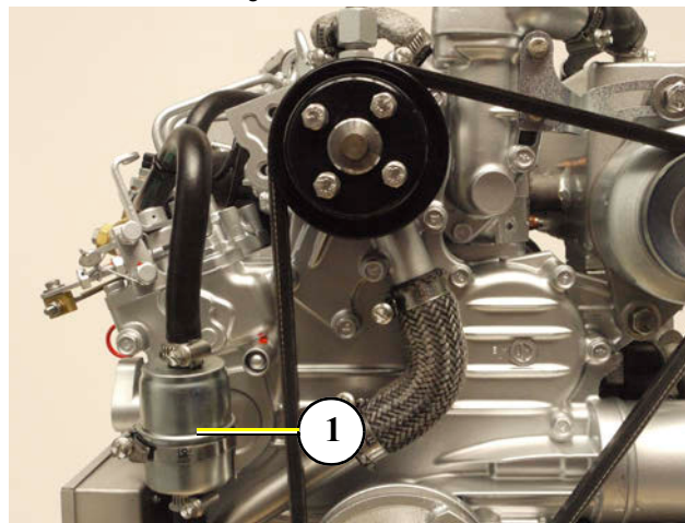
Fig. 10.4.2-1: Fuel filter
