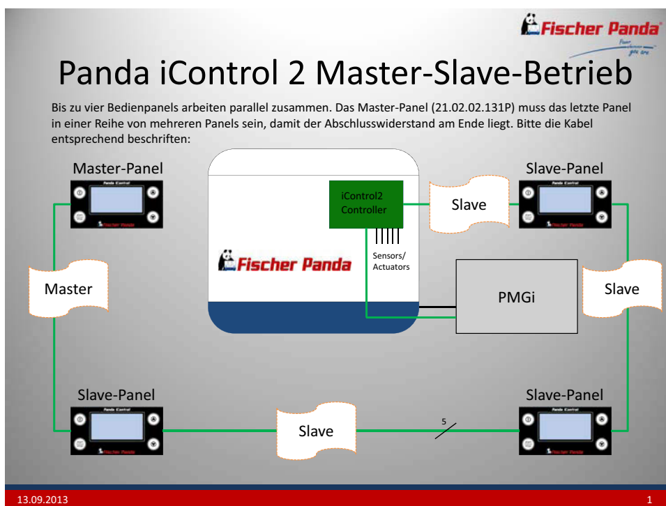
Fig. 15.5-1: Master Slave Schema
