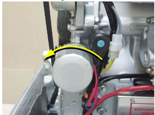
Fig. 8.11-3: Ölfilter
