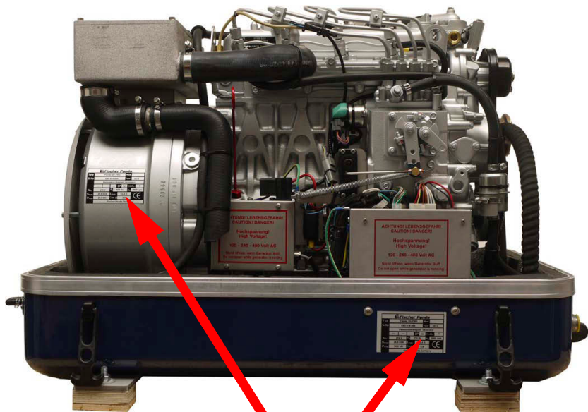
Fig. 5.1-1: Panda 25i PMS Generator
