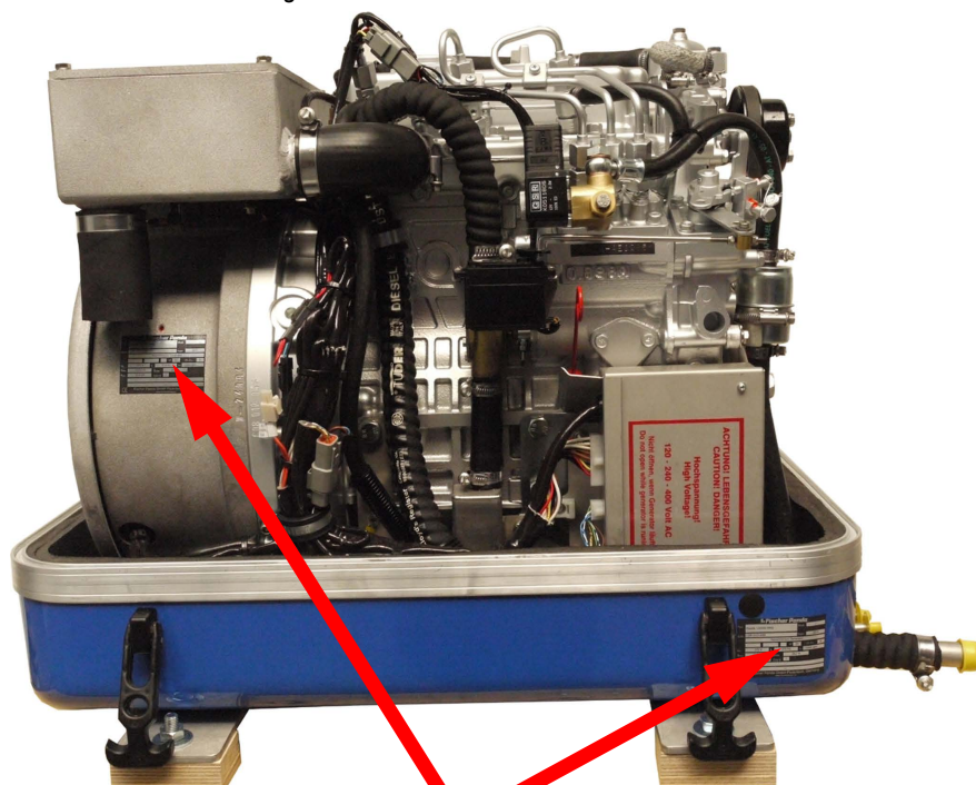
Fig. 7.1-1: Panda 15000i PMS Generator
