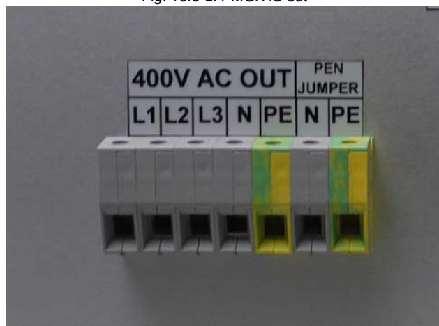
Fig. 13.5-3: PMGi AC out
